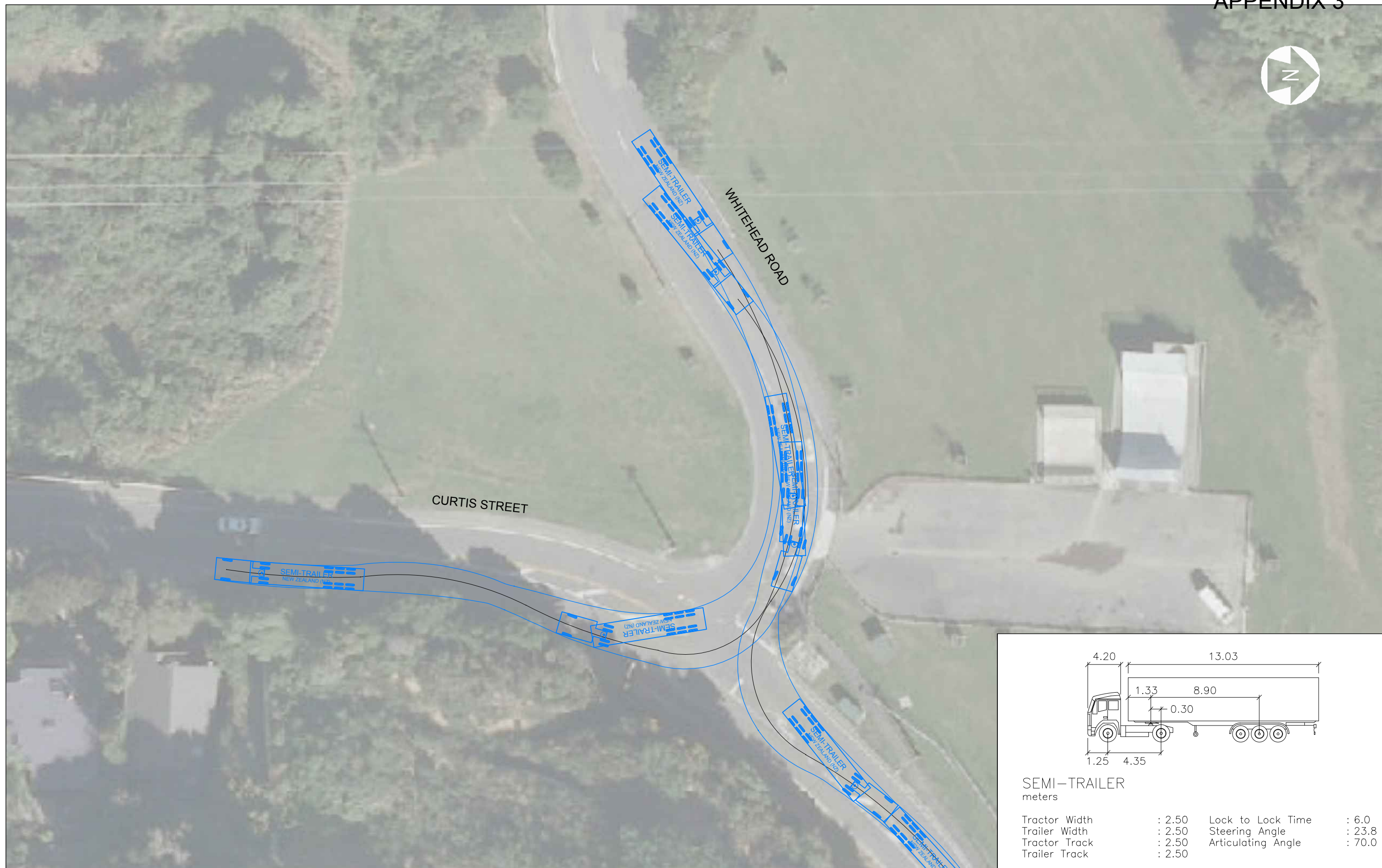
WHITEHEAD ROAD TO CURTIS STREET SEMI-TRAILER TRACKING PATHS
