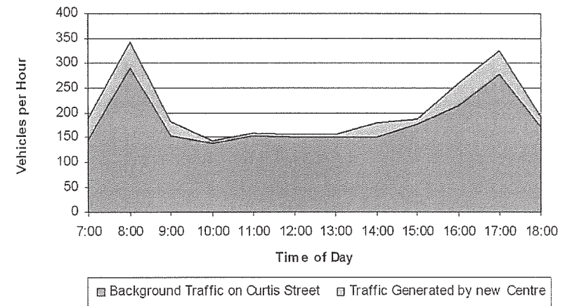
Expected Traffic Volumes on Curtis Street
