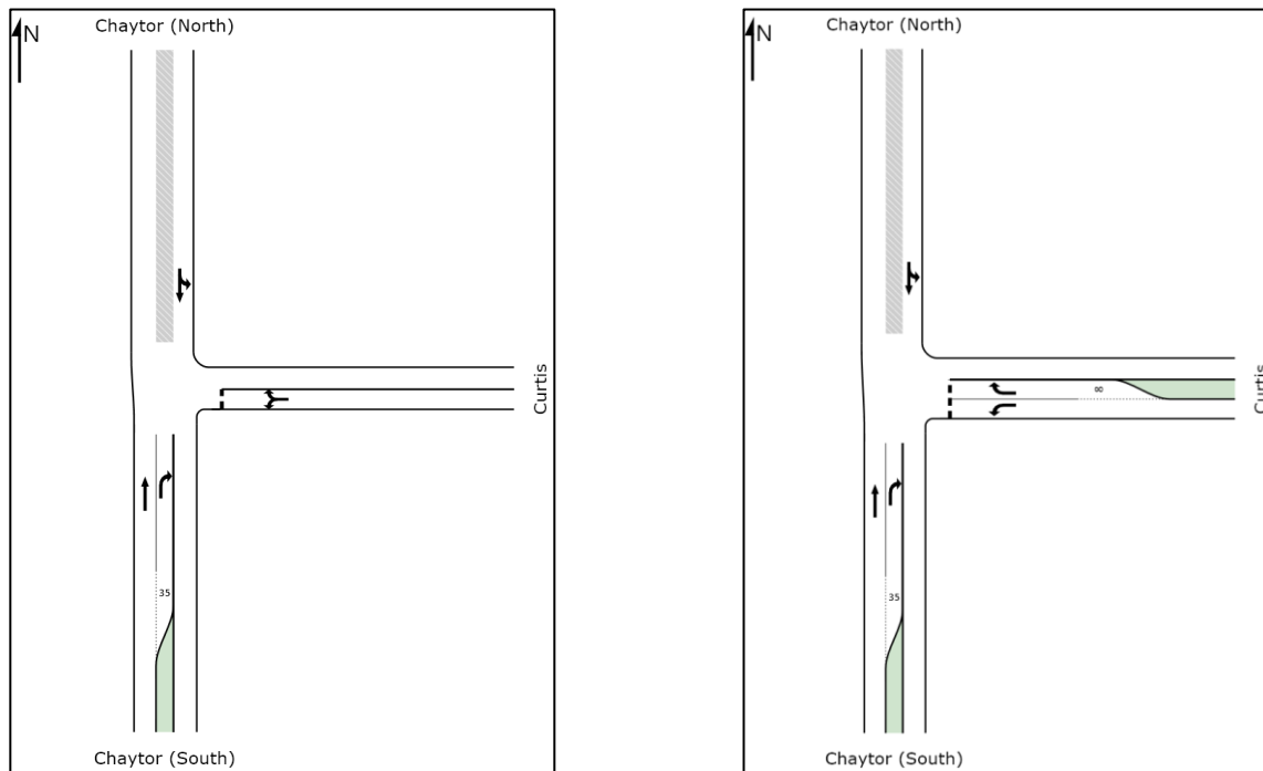
Figure 6-2 Curtis / Chaytor Intersection Mitigation Measures
