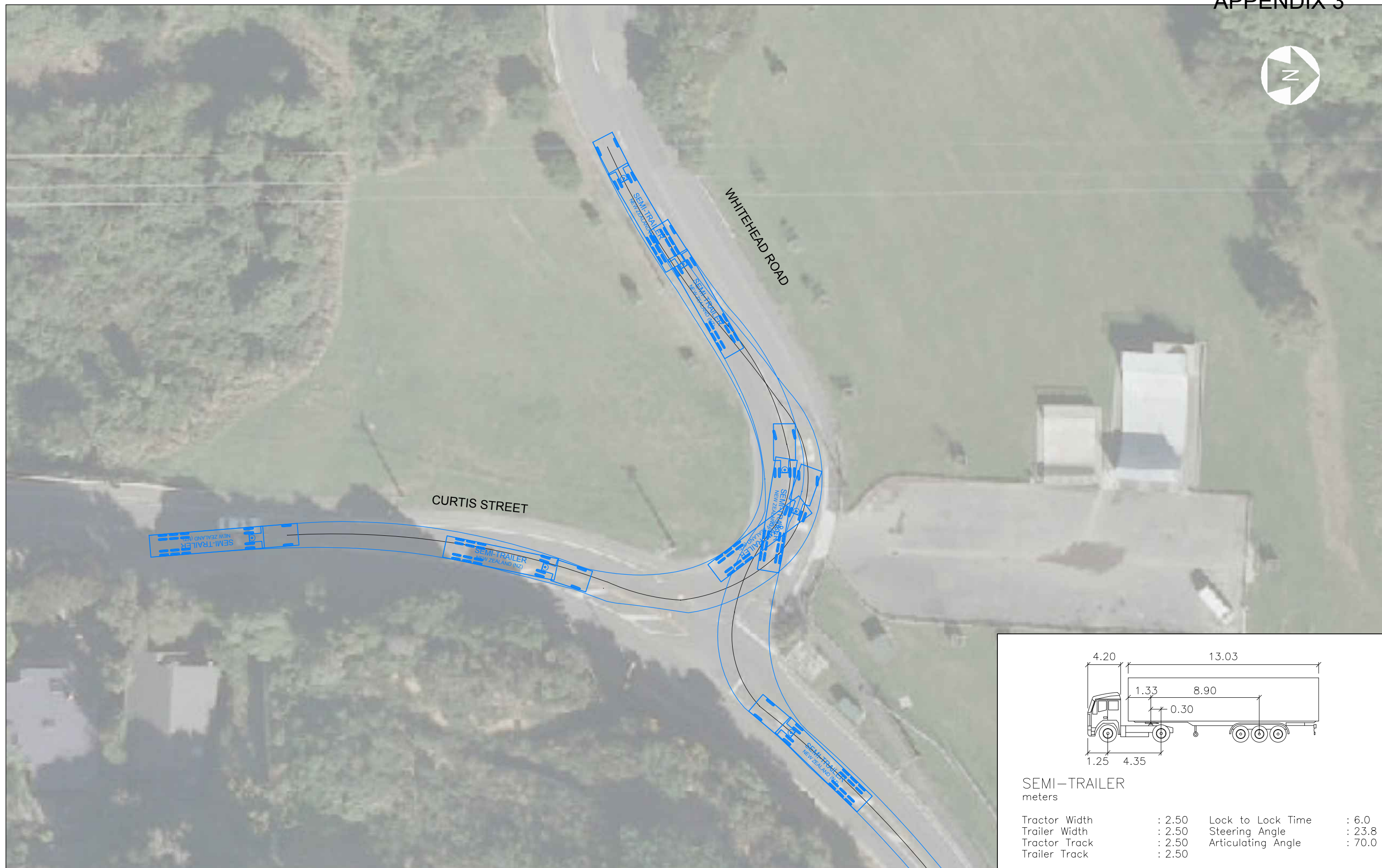
CURTIS STREET TO WHITEHEAD ROAD SEMI-TRAILER TRACKING PATHS
