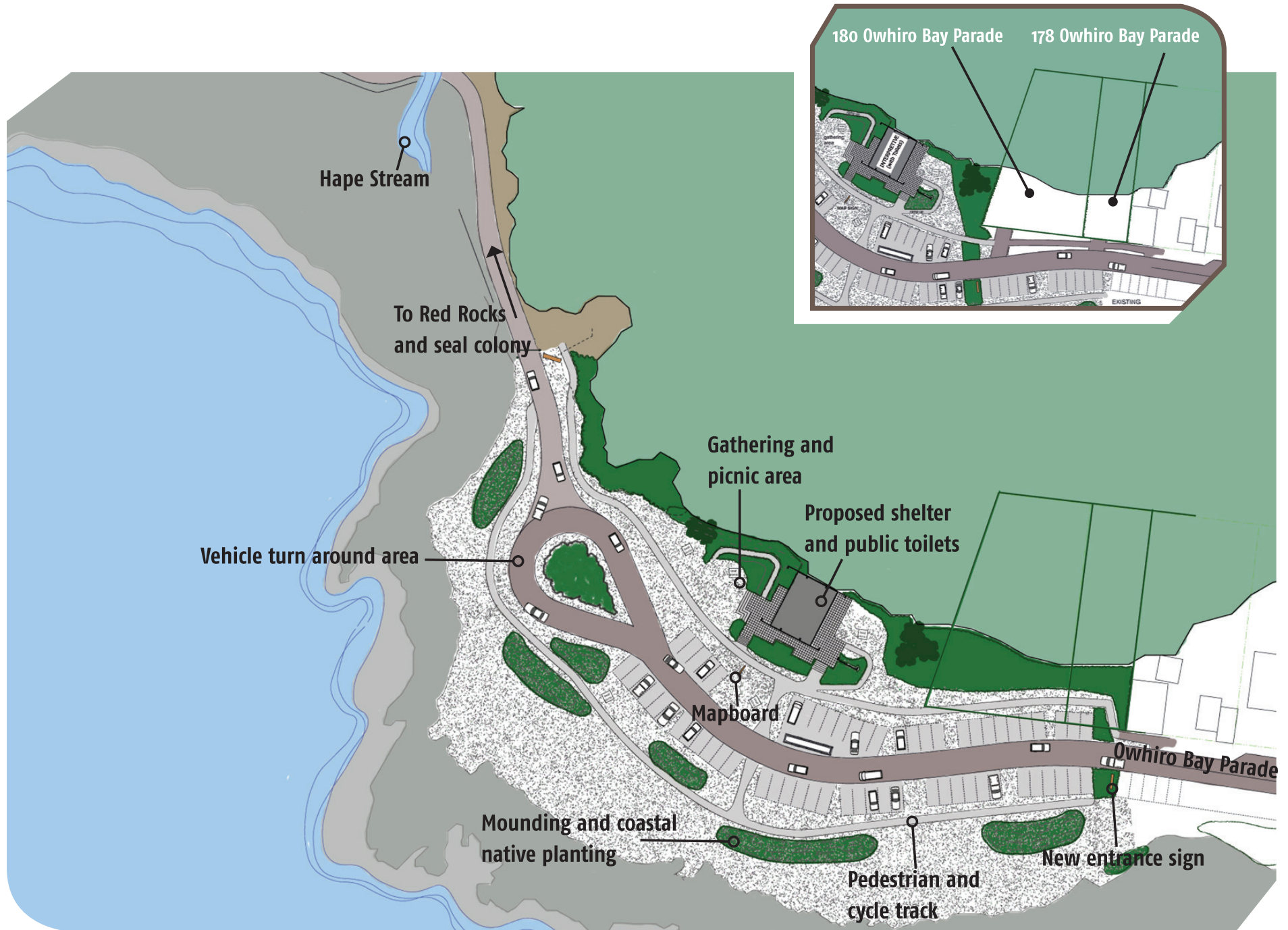
Owhiro Bay Entrance Concept Plan showing the proposed layout including the two sections. The insert above shows the layout if the sections are sold.
