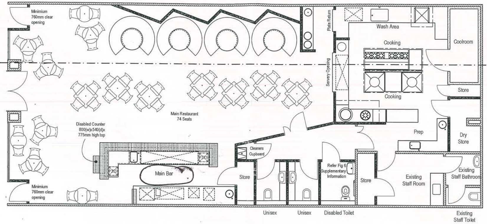
PROPOSED LAYOUT PLAN 1:100 Scale
