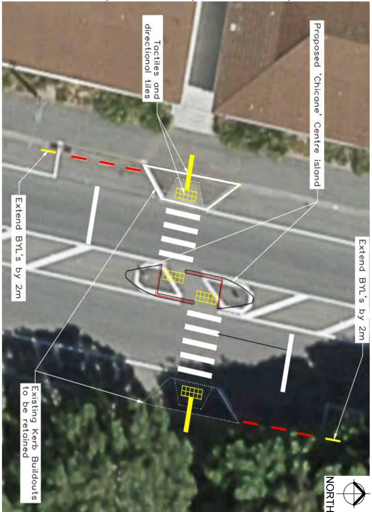
Attachment 1: Indicative layout Pedestrian Facility Adelaide Road, Berhampore
